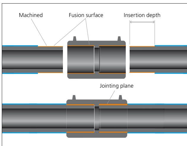
8.44 Principle of electrofusion welding
