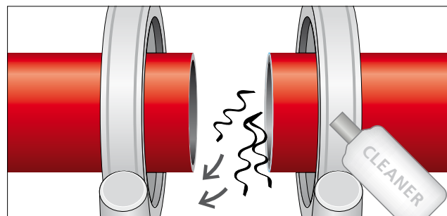
8.40 Remove chips and shavings in the jointing area and clean the fusion surfaces with PE cleaner
