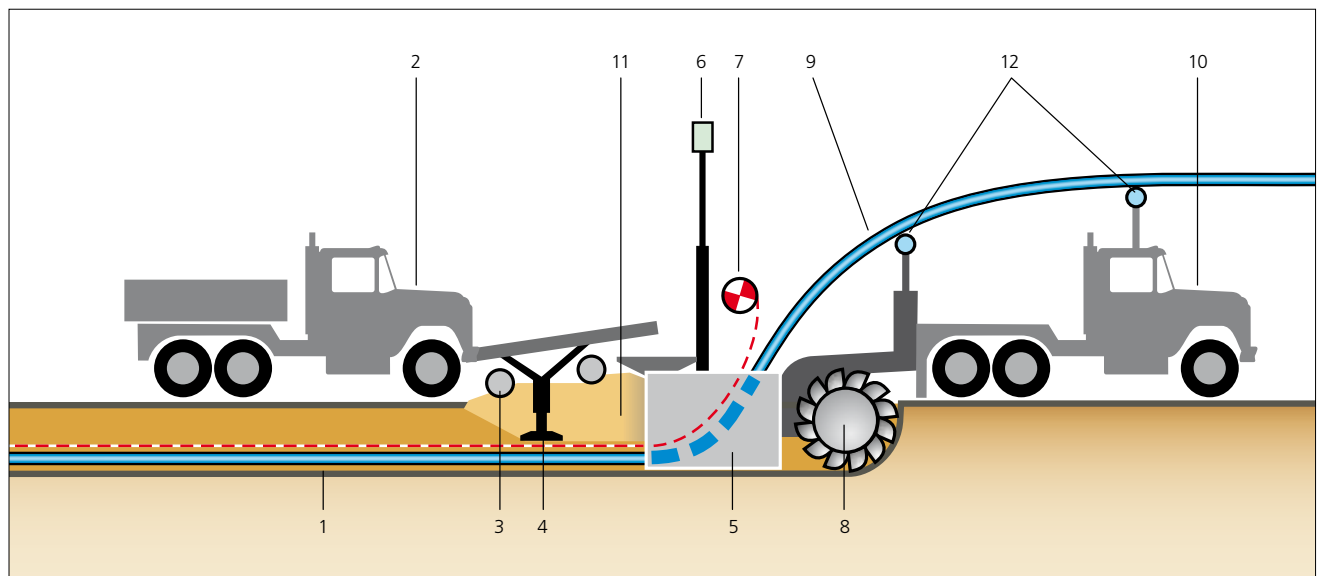
8.29 Narrow trenching | 1 trench bottom | 2 backfill and compaction unit | 3 axial screw conveyors | 4 compactor | 5 laying box | 6 laser receiver | 7 utility marking tape | 8 milling disc or cutter chain | 9 EMDS conduit | 10 trenching and laying unit | 11 extracted material (spoil) | 12 piping guides
